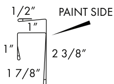
F-J TRIM
