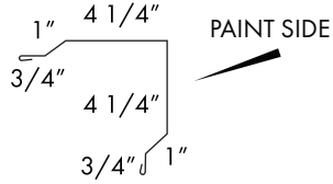
RIDGE CAP
