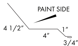
J-J TRIM
