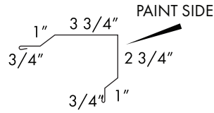
RAKE TRIM
