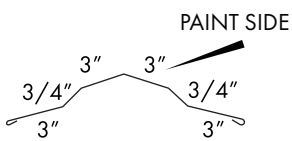
UPPER GAMBREL
