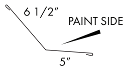
END WALL
