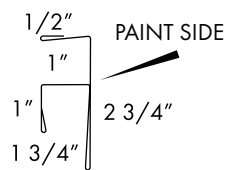
J-J TRIM
