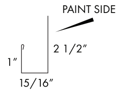
RAT GUARD
