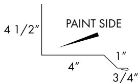
F-J TRIM
