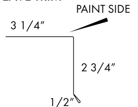
EAVE TRIM
